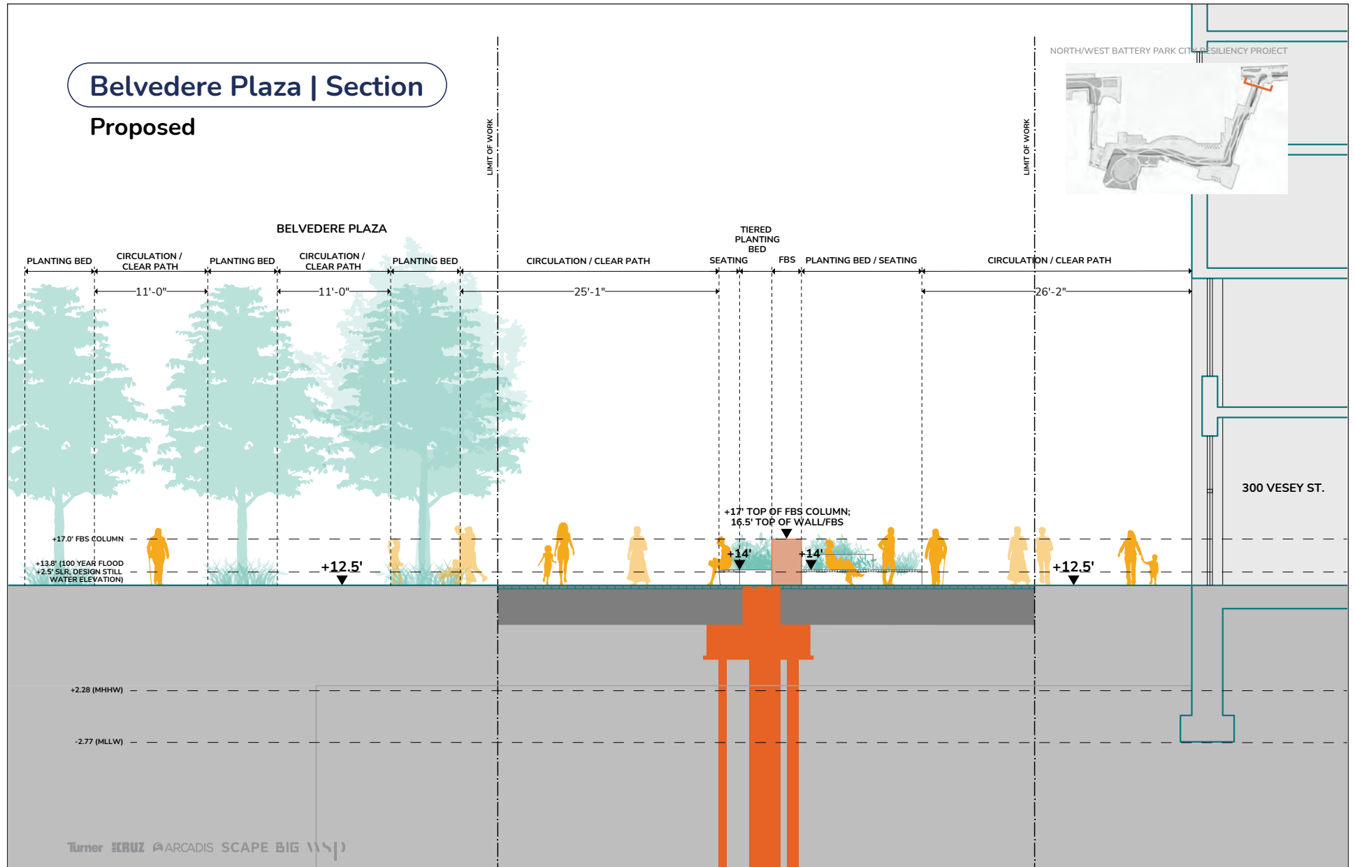
Reach 5 Proposed Section - Belvedere Plaza Figure 1-16e
