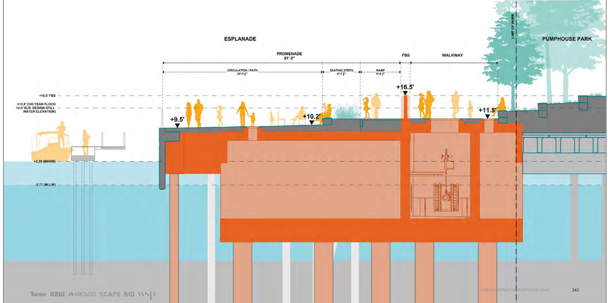
Reach 5 Proposed Section - Pumphouse Park Figure 1-16g
