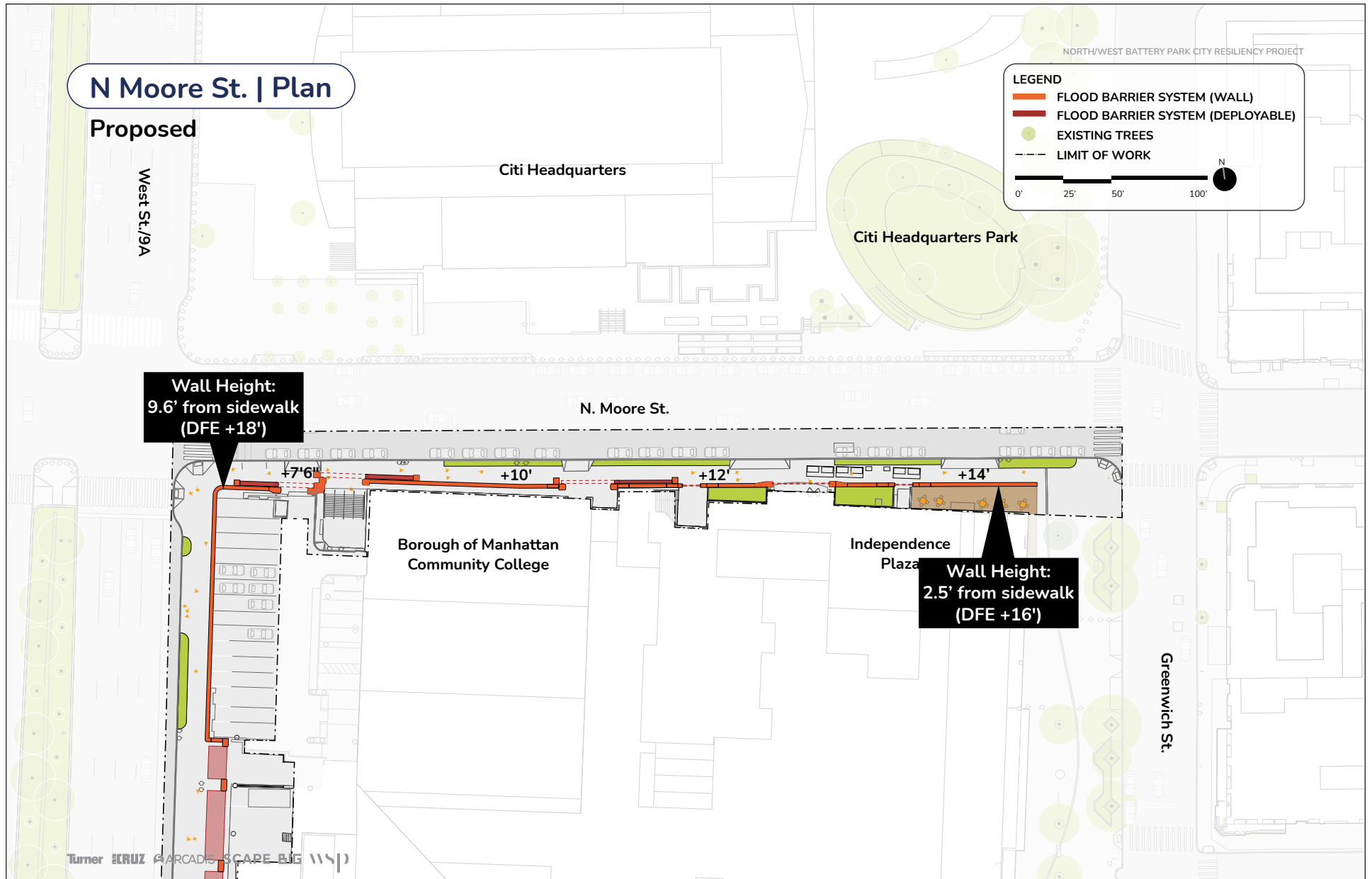
Reach 1 Proposed Site Plan - North Moore Street Figure 1-12b
