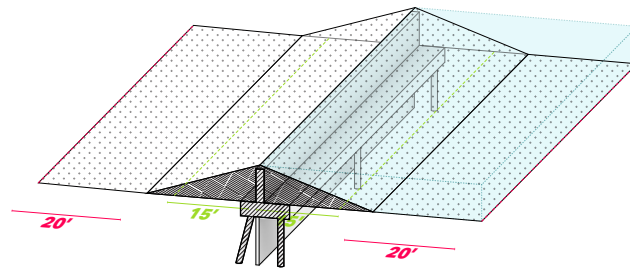
NON-STRUCTURAL BERM
