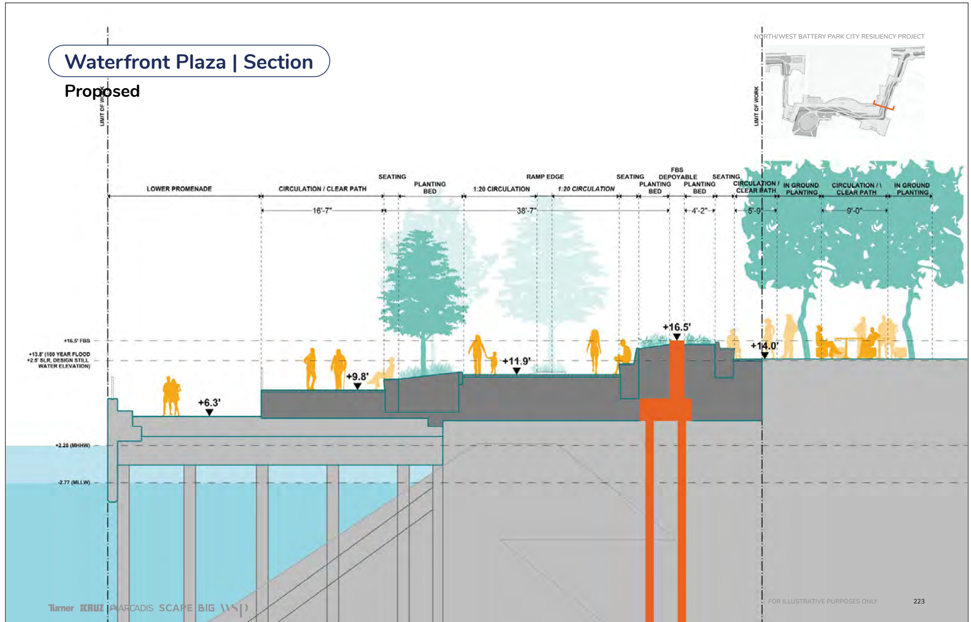
Reach 5 Proposed Section - Waterfront Plaza Figure 1-16f
