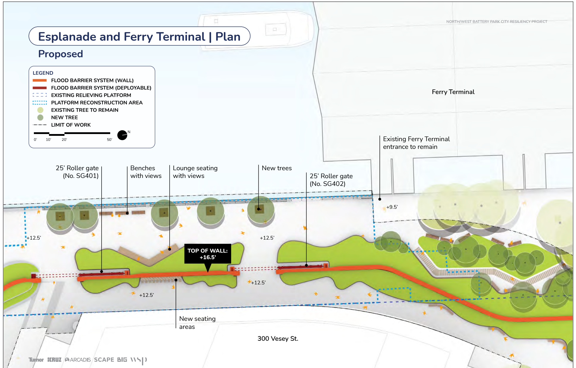
Reach 4 Proposed Site Plan - Esplanade and Ferry Terminal
