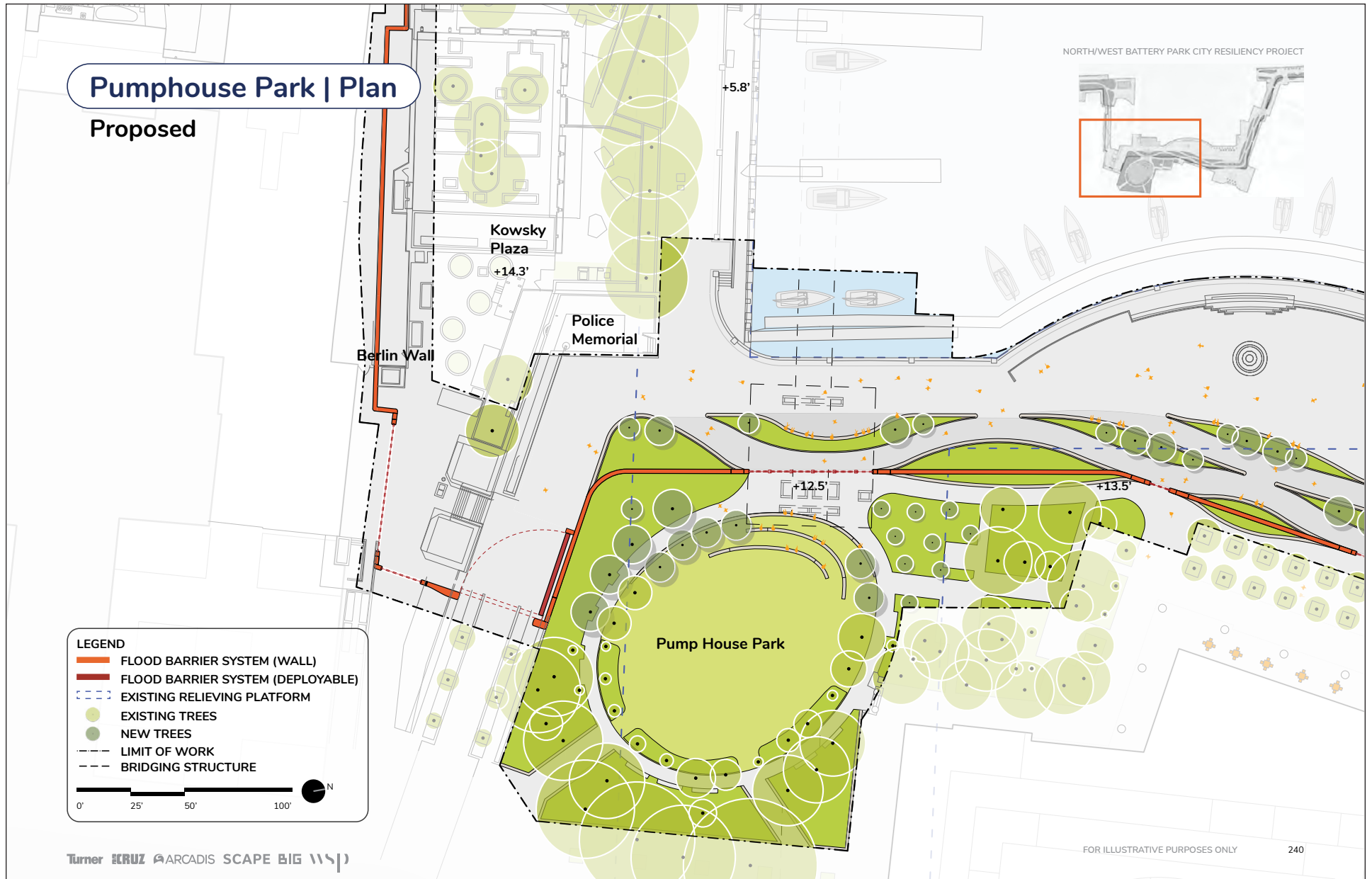
Reach 5 Proposed Site Plan - Pumphouse Park Figure 1-16c
