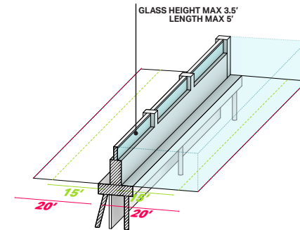
GLASS-TOPPED WALL
