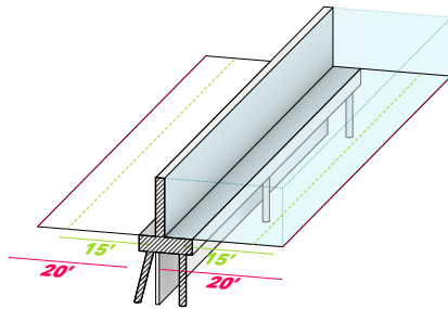
FLOODWALL
