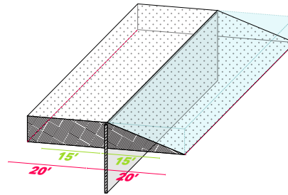
CONCEALED FLOODWALL
