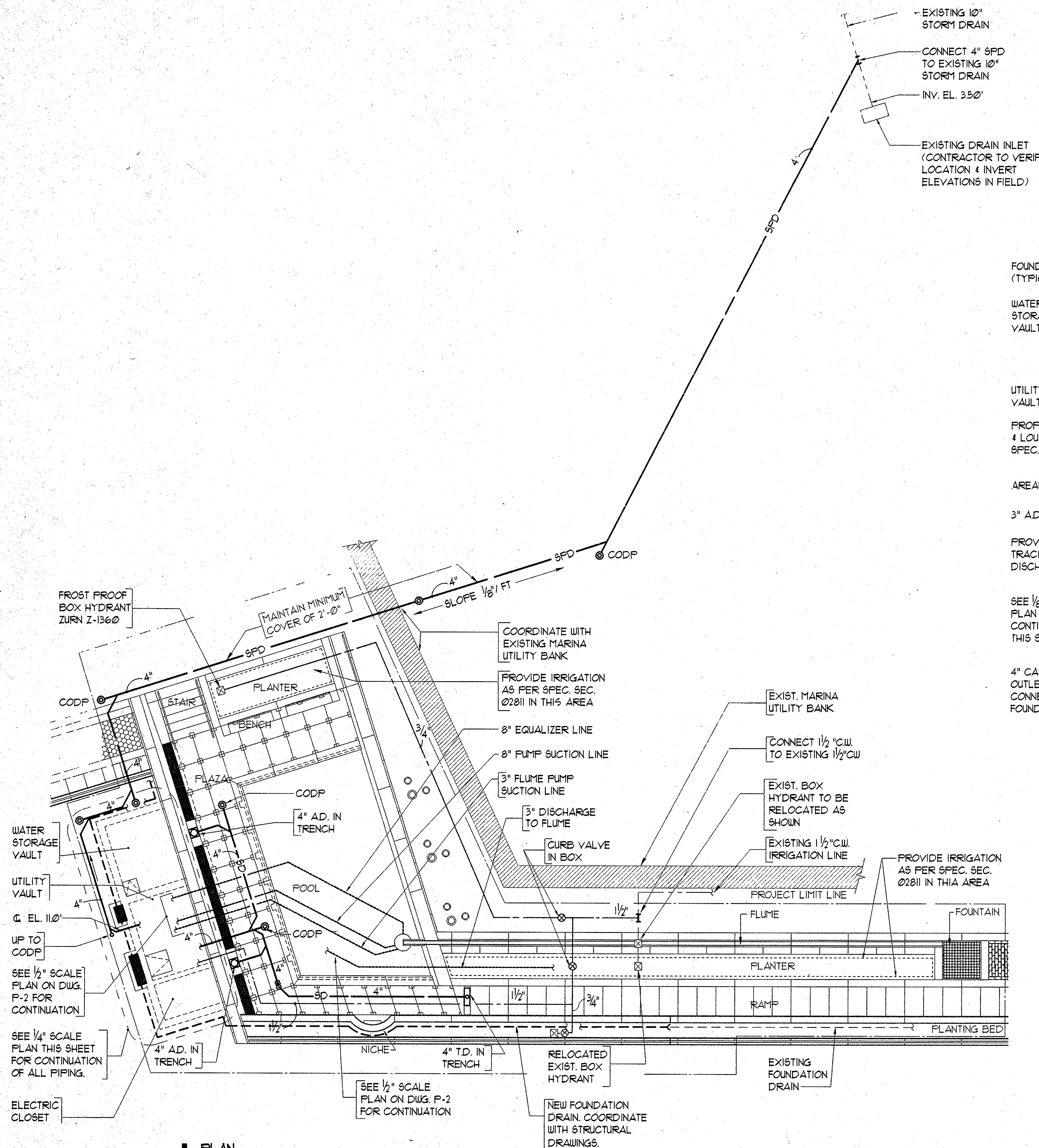
1 PLAN 1/8" = 1'-0"
