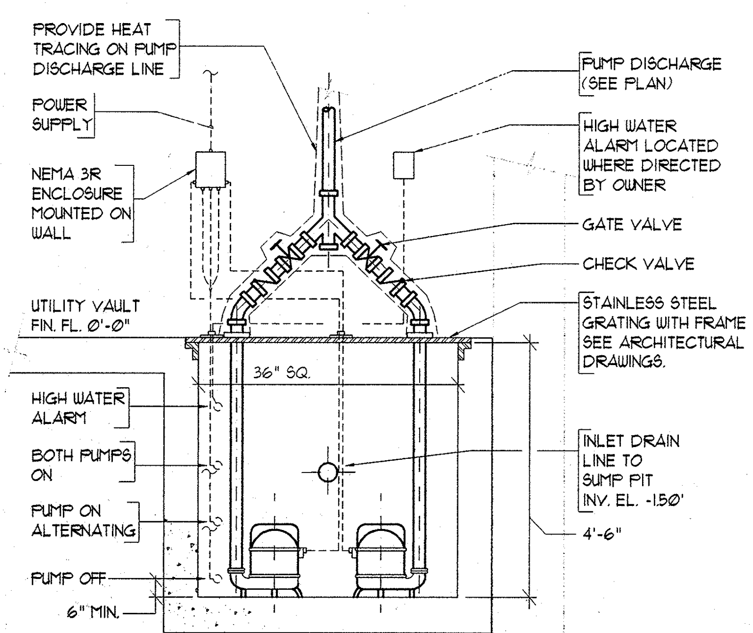
3 SUMP PUMPS AND PIT DETAIL NOT TO SCALE
