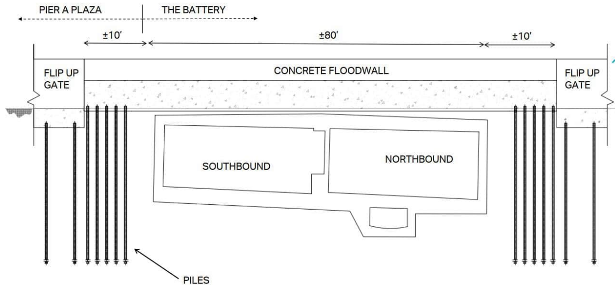
Figure 2.2-17: Exposed Floodwall Foundation over the Battery Park Underpass
