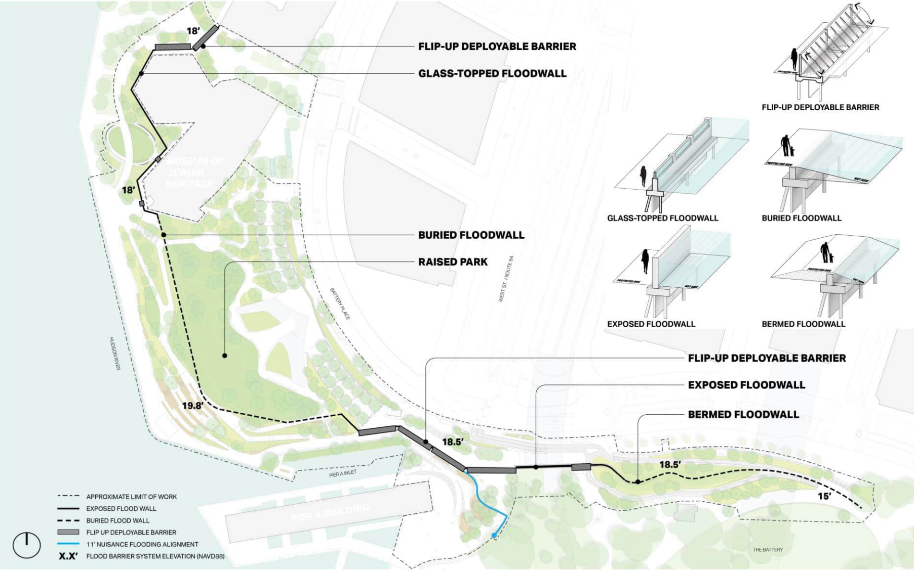
Figure ES-4: SBPCR Project Flood Alignment and DFEs
