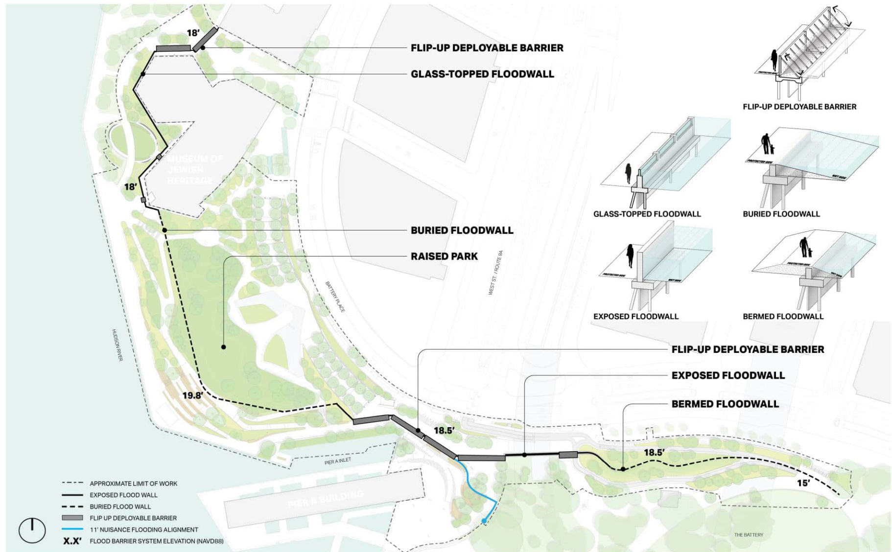
Figure 3.4-1: SBPCR Project Flood Alignment and DFEs
