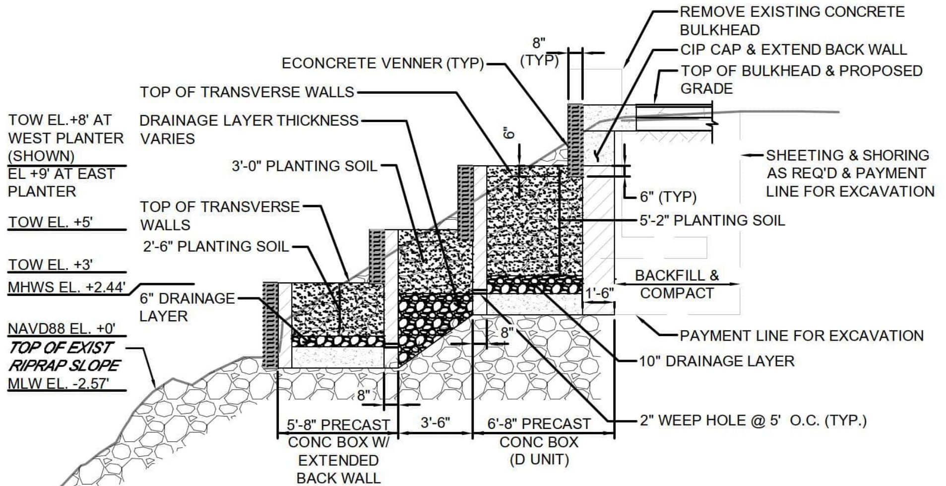
Figure 3.7-2: Shoreline with Planting Shelves at 3, 6 and 8 Feet
