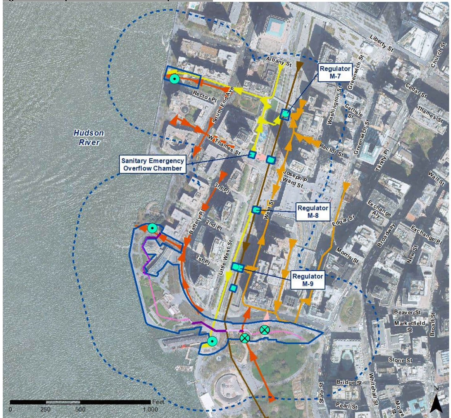
Figure 3.8-3: Proposed Water and Sewer Improvements
