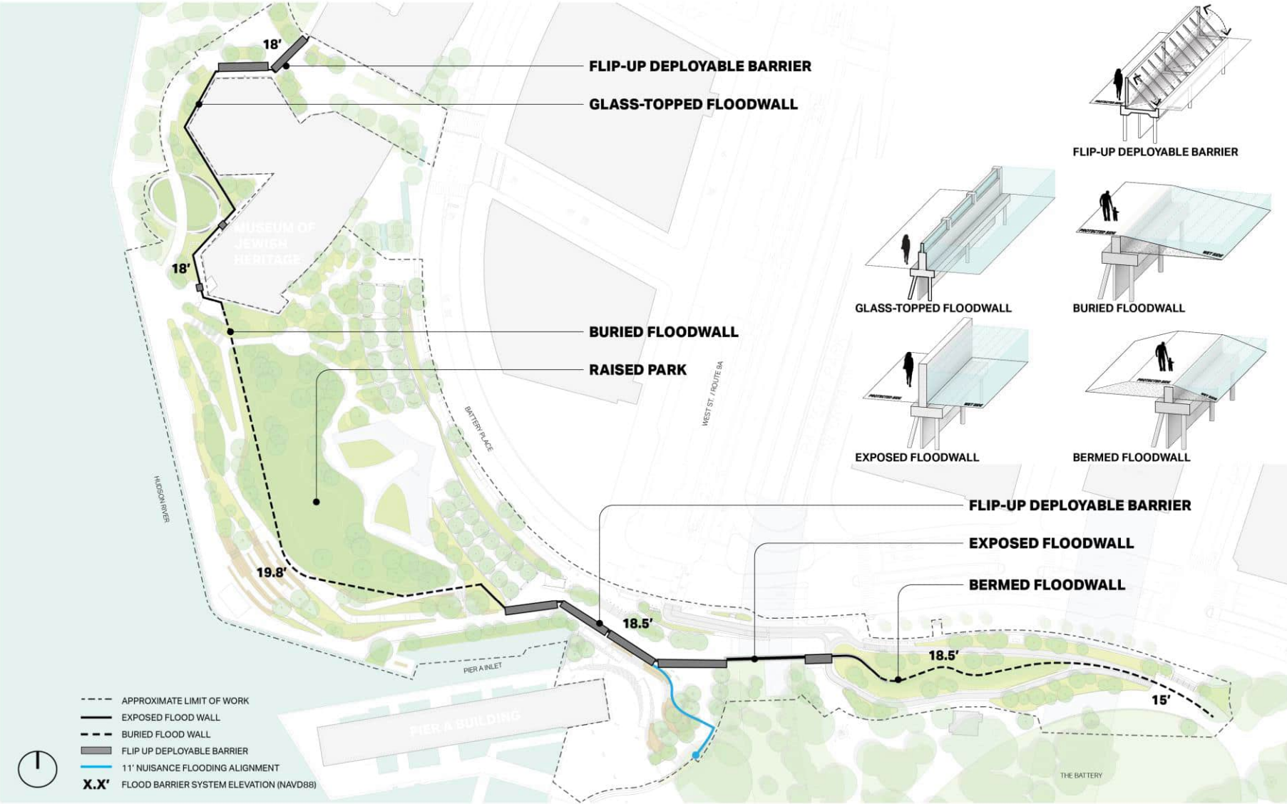
Figure 1.3-1: SBPCR Project Flood Alignment
